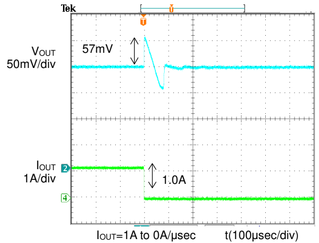
Figure 12. Transient Response (1.0A to 0A) C_{OUT}=22\mu F , C_{FB}=1000pF
