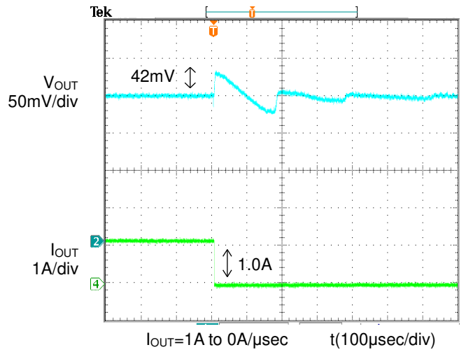
Figure 10. Transient Response (1.0A to 0A) C_{OUT}=100\mu F , C_{FB}=1000pF
