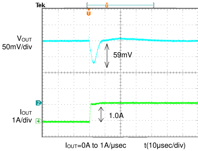
Figure 9. Transient Response (0A to 1.0A) C_{OUT}=22\mu F , C_{FB}=1000pF
