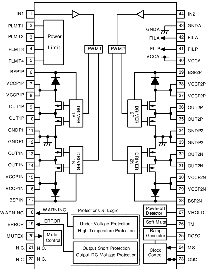
Fig. 28 Pin Assignment Diagram
