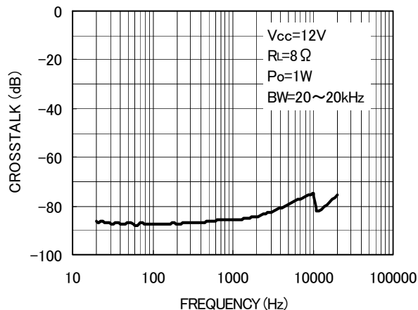
Fig. 4 Crosstalk - Frequency
