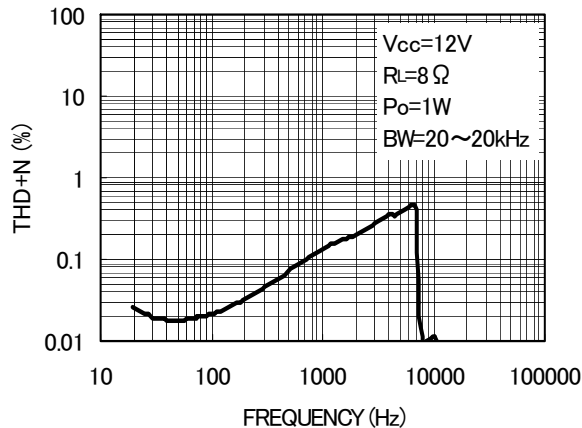
Fig. 2 THD+N - Frequency
