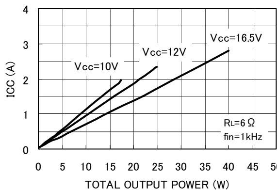
Fig. 22 Current consumption - Output power
