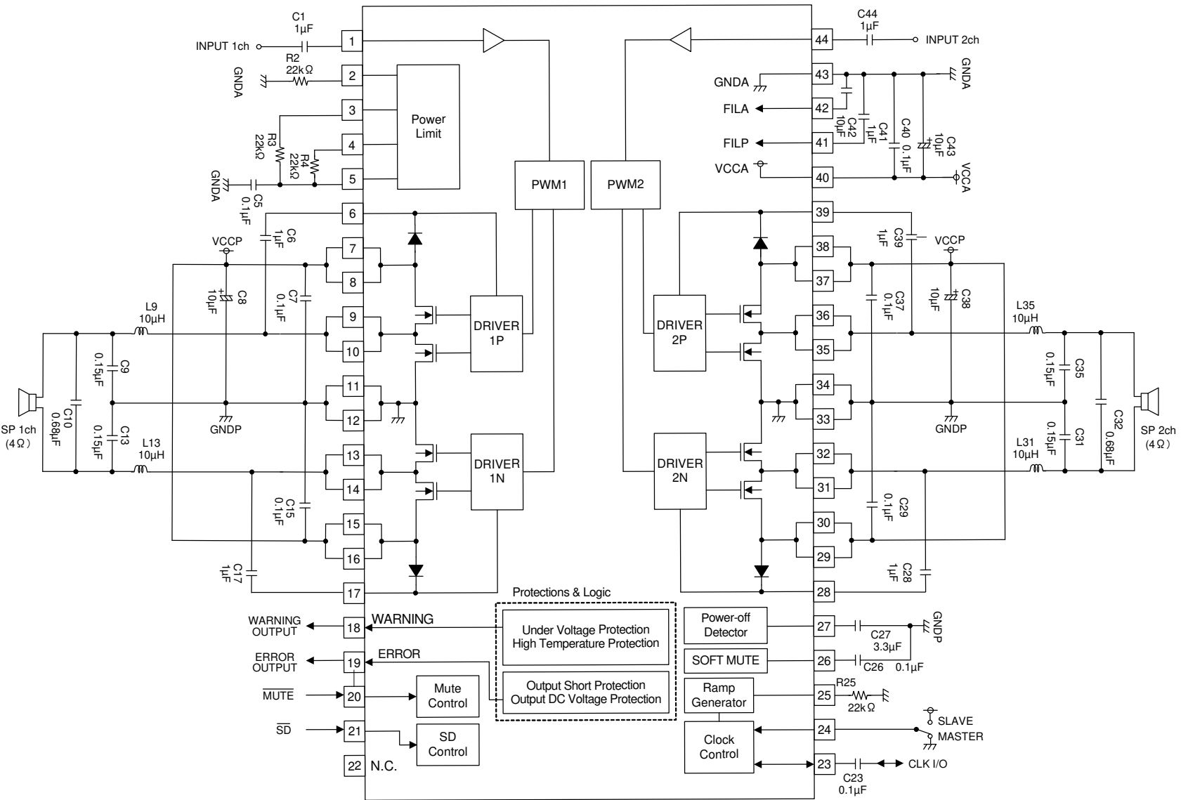
Fig. 30 Circuit Diagram of Stereo Operation with 4Ω Load
