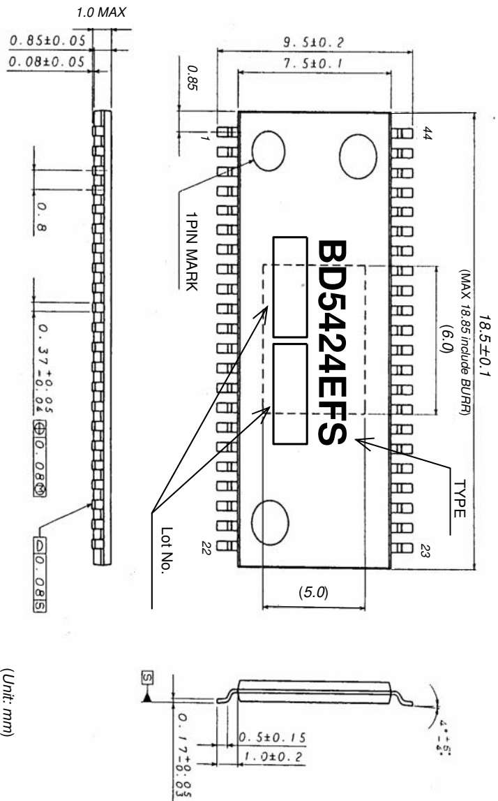
Fig. 29 Outer Dimensions and Inscriptions of HTSSOP-A44 Package
