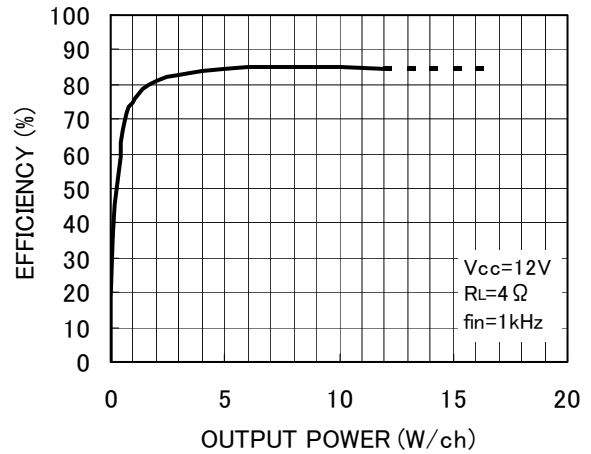
Fig. 25 Efficiency - Output power
