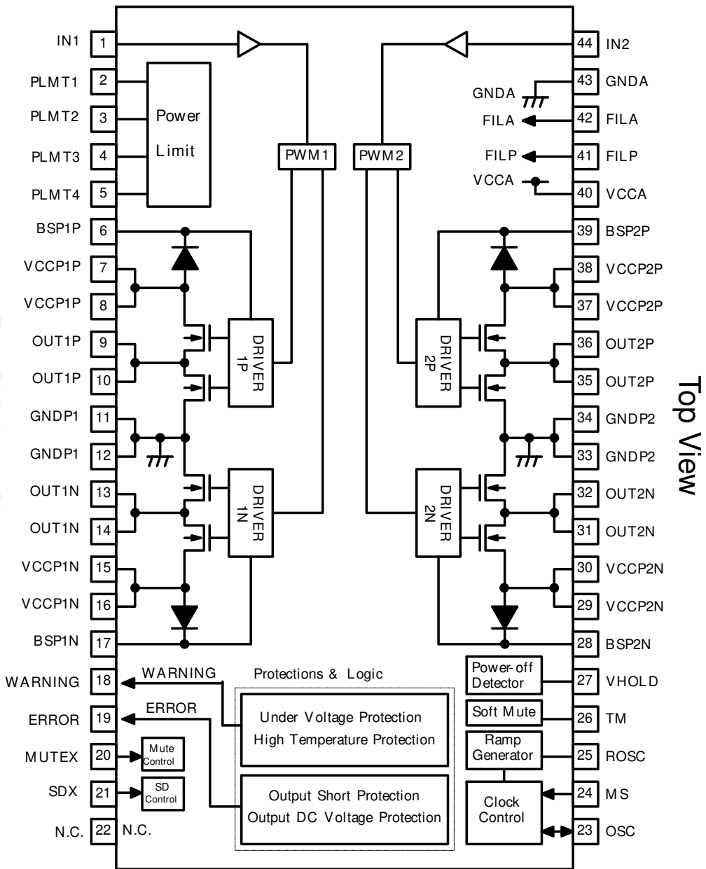
Fig. 28 Pin Assignment Diagram
