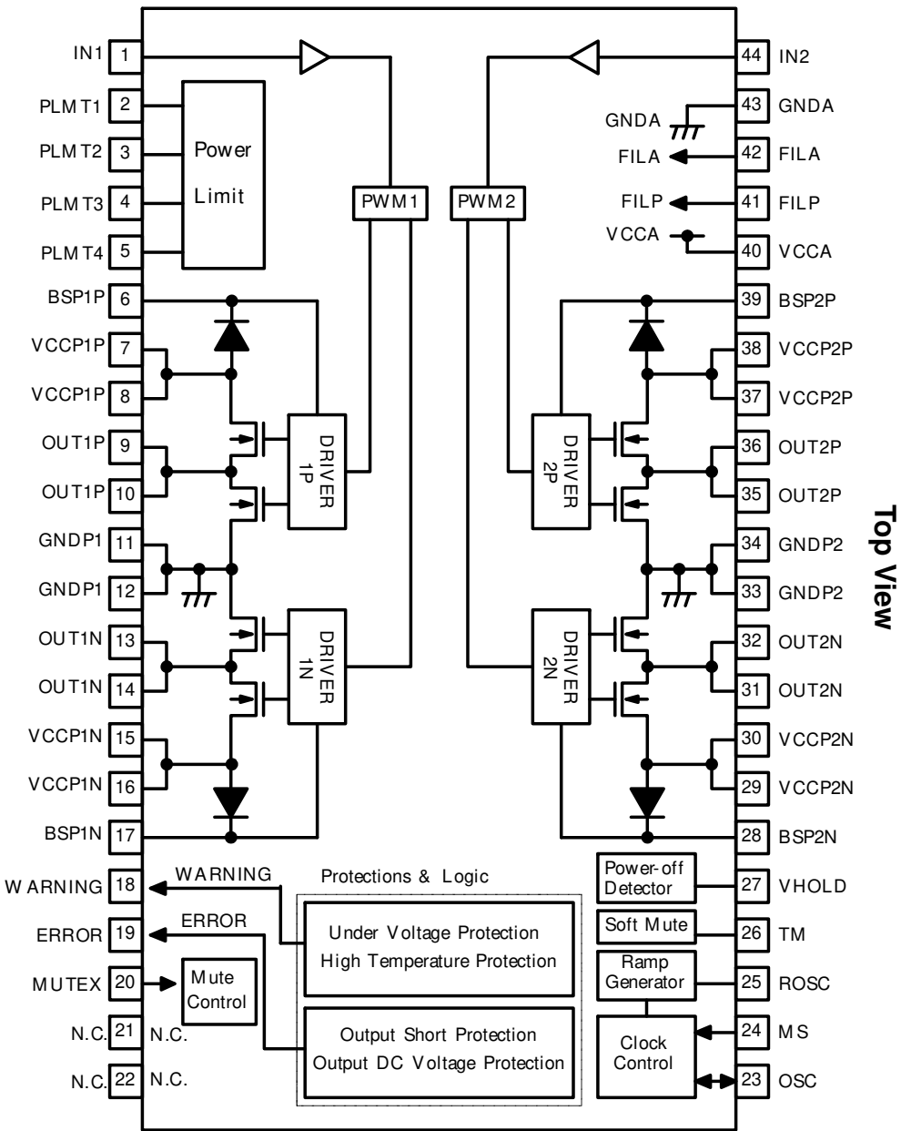
Fig. 23 Pin Assignment Diagram
