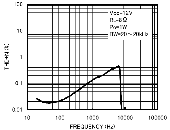
Fig. 2 THD+N - Frequency
