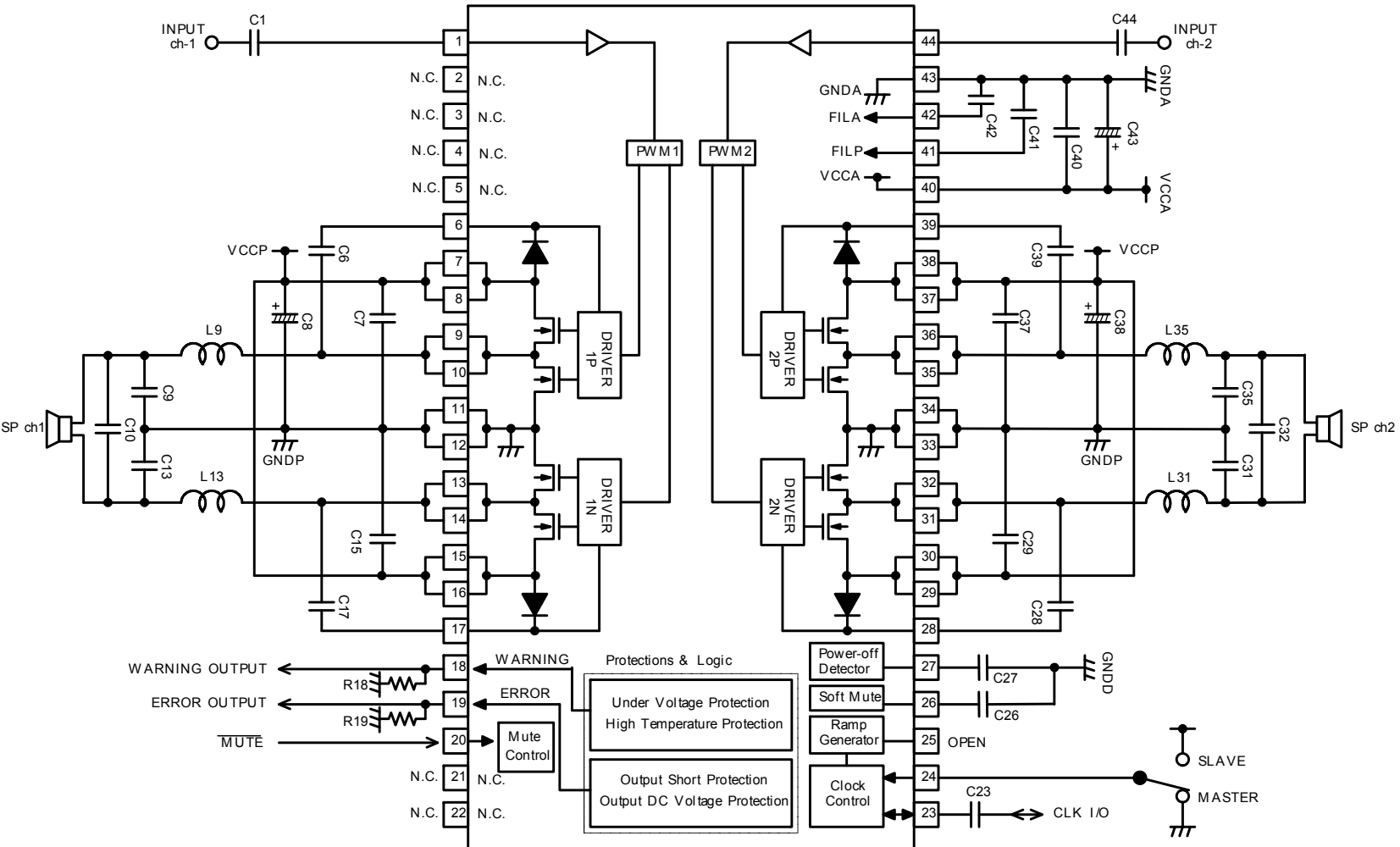
Fig. 24 Circuit Diagram of Stereo Operation with 8Ω Load
