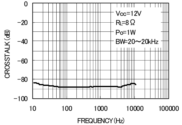
Fig. 4 Crosstalk - Frequency
