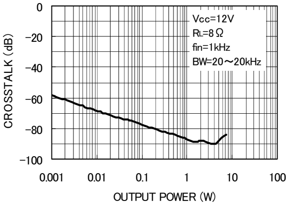
Fig. 5 Crosstalk - Output power
