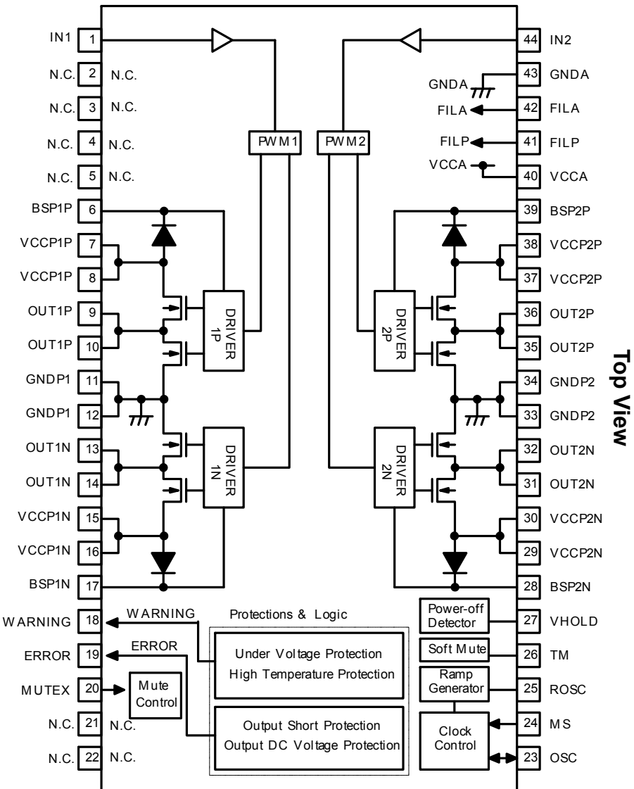
Fig. 22 Pin Assignment Diagram
