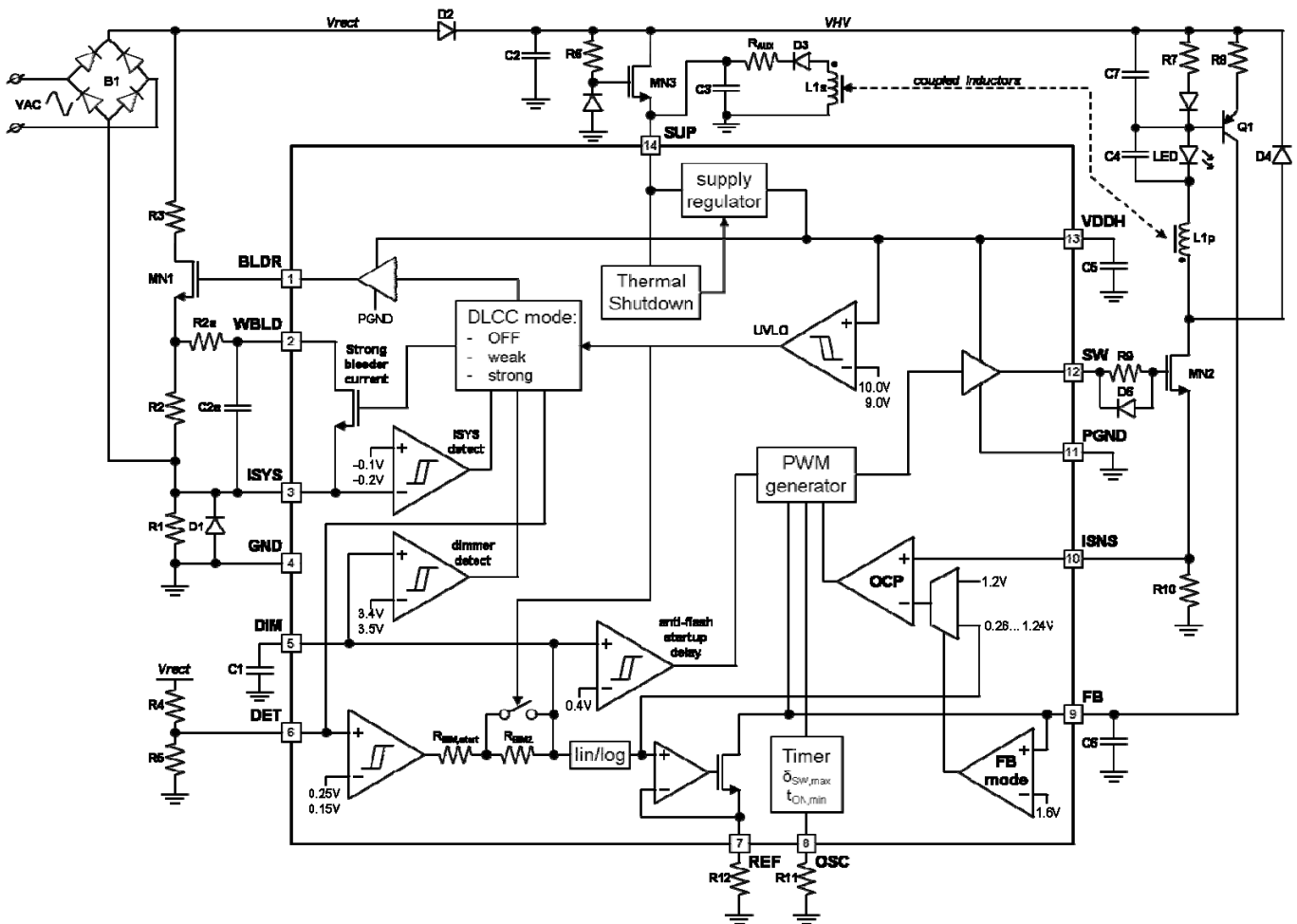
Figure 4. Block diagram
