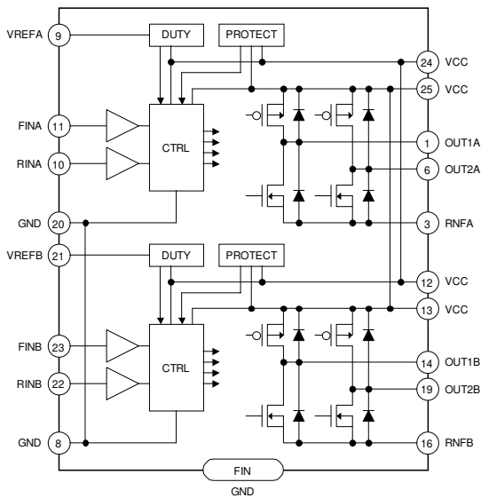
Fig.7 BD6236FP
