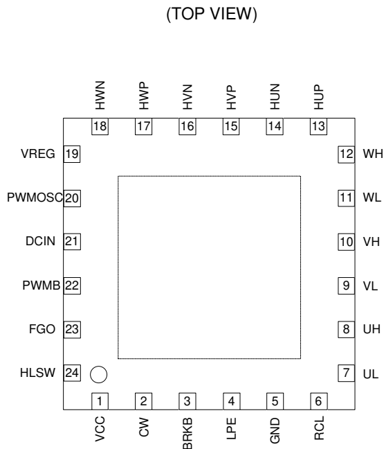
Figure 4. Pin Configuration
