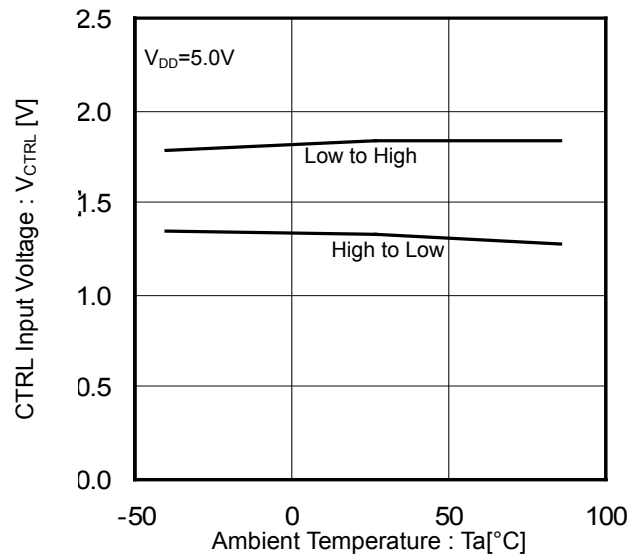
Figure 8. CTRL Input Voltage vs Ambient Temperature
