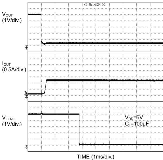
Figure 33. Over-Current Response Output Short Circuit at Enable
