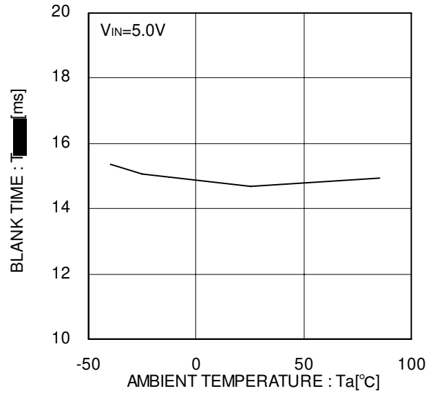
Figure 26. Blanking time
