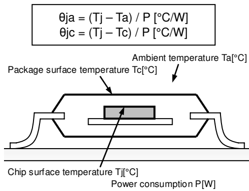
Fig.34 Thermal resistance
