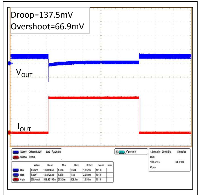
Figure 24. Load Transient Response (VIN=3.6V, VOUT=1.8V, IOUT=1uA↔500mA, tr=tr=1μs)
