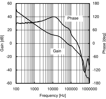
Fig.43 Frequency response 9 (VCC=10V, Io=900mA)
