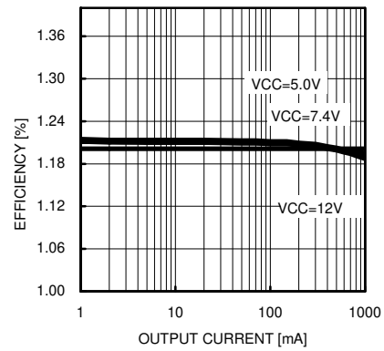
Fig.34 Load regulation (VOUT = 1.2 V)
