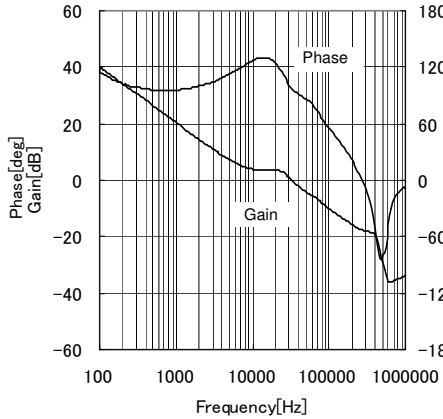
Fig.25 Frequency response 2 (VCC=6.0V, Io=250mA)
