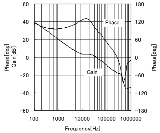
Fig.29 Frequency response 6 (VCC=6.0V, Io=500mA)
