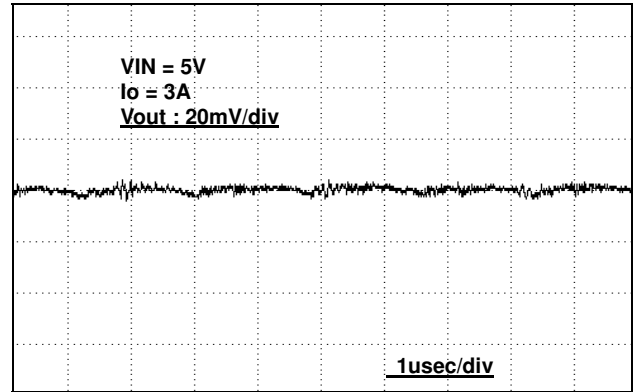
Fig.8 Output ripple
