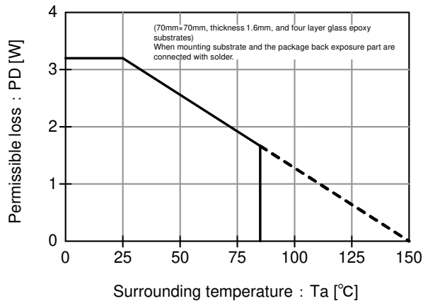
Fig. 1 heat decrease curve
