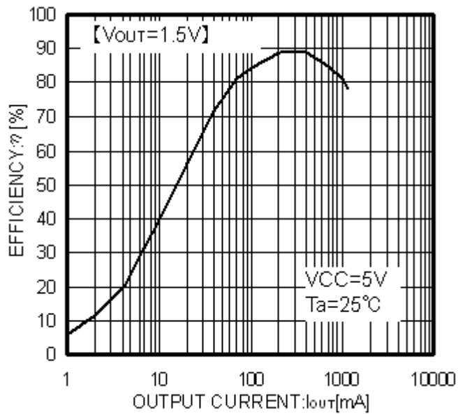
Fig.8 Efficiency
