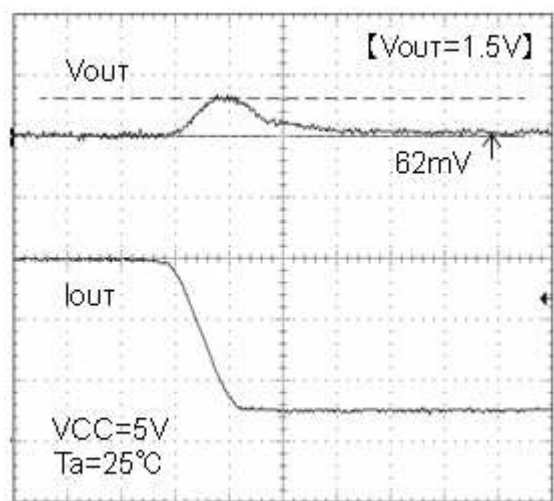
Fig. 17 Transient response Io=600→100mA(10μs)
