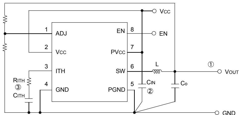
Fig.33 Layout diagram
