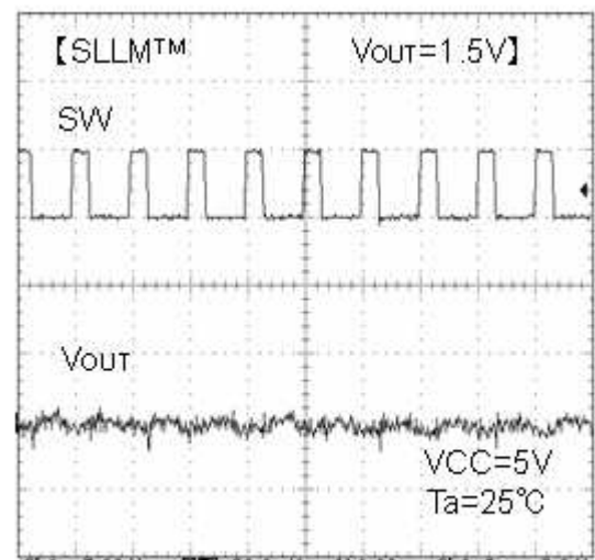
Fig.15 SW waveform
