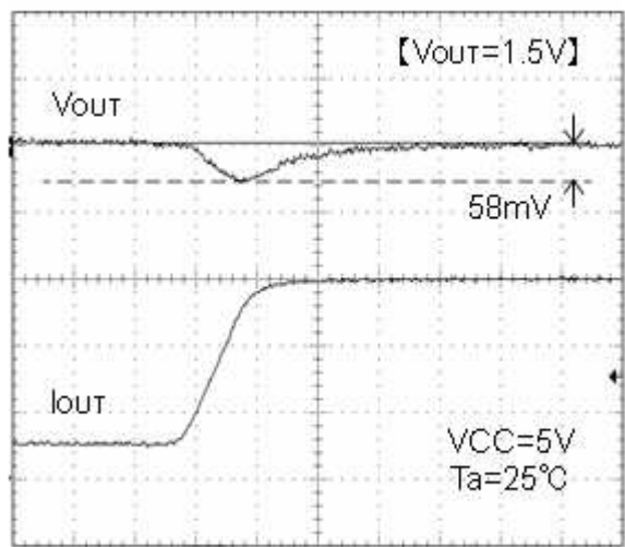
Fig. 16 Transient response Io=100→600mA(10μs)
