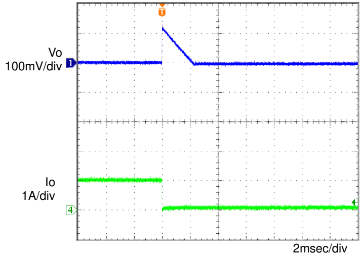
Figure 8. Transient Response (1.0→0A) C_o=1\mu F, T_a=105^\circ C
