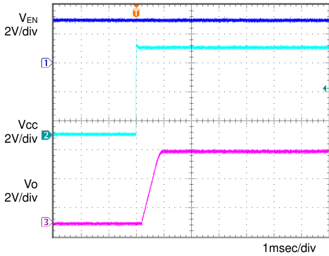
Figure 9. Input sequence 1 C_o=1\mu F, T_a=-40^\circ C
