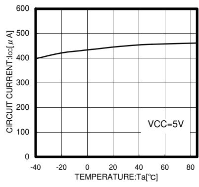
Fig.13 Ta – Icc
