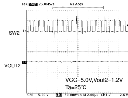
Fig.19 SW2 wave form ( I_{o2}=1.5A )
