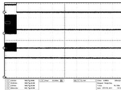
Fig.29 Stop Waveform
