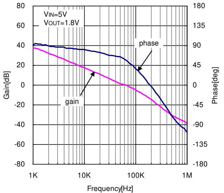
Figure 25. Closed Loop Response (VIN=5V, VOUT=1.8V, IOUT=1A, L=2.2µH, COUT=Ceramic 44µF)
