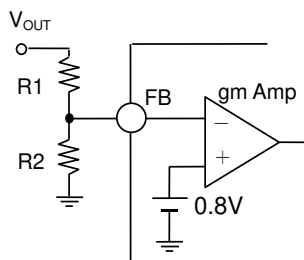
Figure 50. Feedback Resistor Circuit
