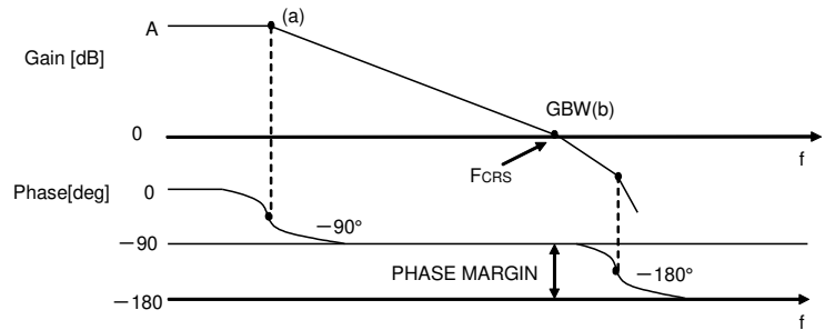
Figure 52. Bode Plot
