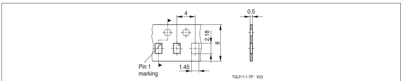
Figure 8-4 Tape Dimensions
