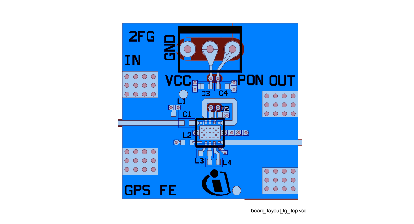
Figure 3 Top View of Application board
