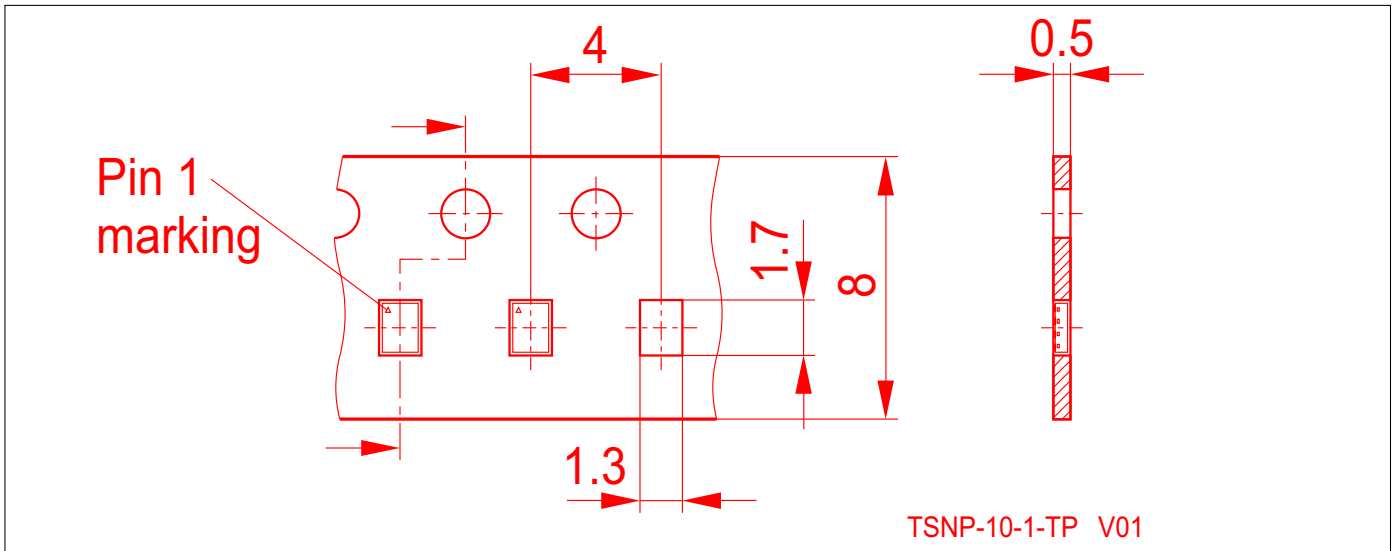
Figure 5: Tape drawing
