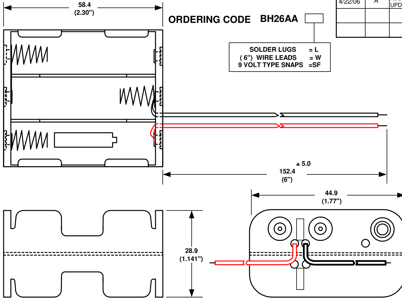
WIRE LEADS SHOWN ABOVE
