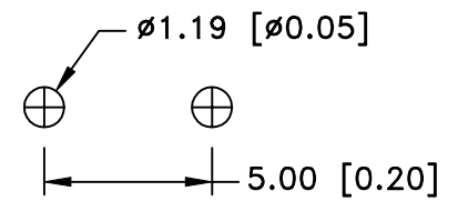
MOUNTING DETAIL
