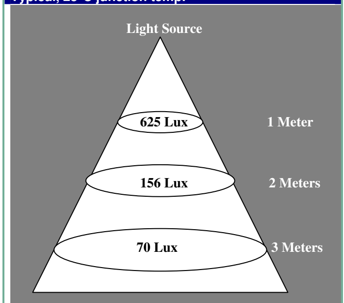
Figure 2 Illuminance Cone – BL-3000 5500K White Typical, 25°C junction temp.
