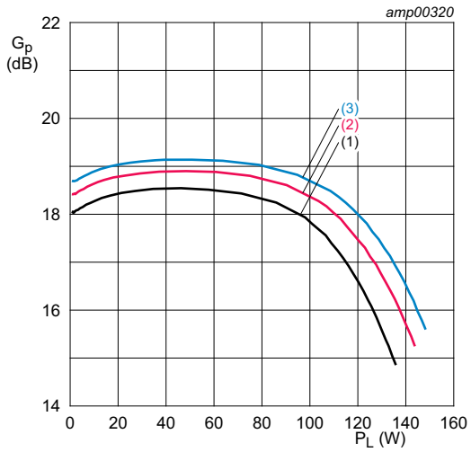
V_{DS} = 28\text{ V}; I_{Dq} = 700\text{ mA}; t_p = 100\text{ }\mu\text{s}; \delta = 10\text{ \%}. (1) f = 1810\text{ MHz} (2) f = 1840\text{ MHz} (3) f = 1875\text{ MHz}
