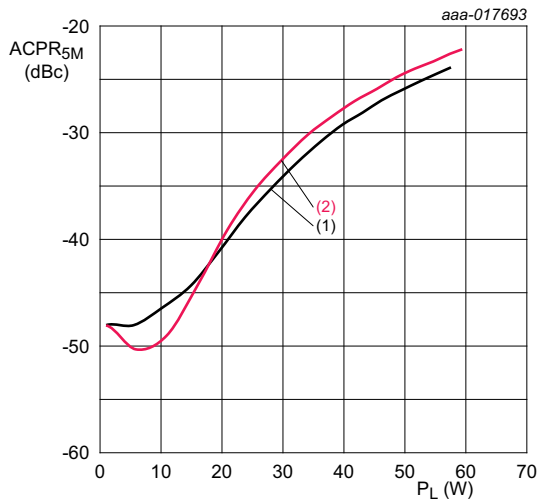
V_{DS} = 28\text{ V}; I_{Dq} = 700\text{ mA}; 5\text{ MHz carrier spacing.} (1) f = 1810\text{ MHz} (2) f = 1875\text{ MHz}
