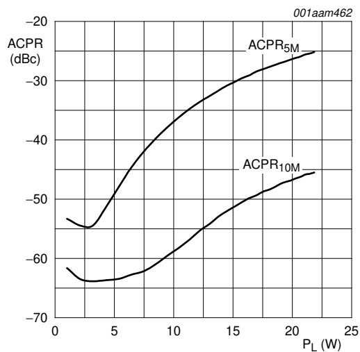
Fig 6. ACPR at 5 MHz and at 10 MHz as function of load power; typical values
