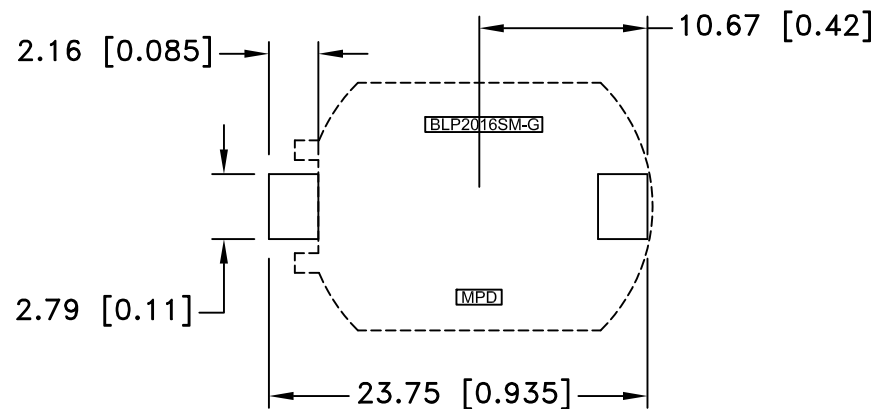
PCB LAYOUT
