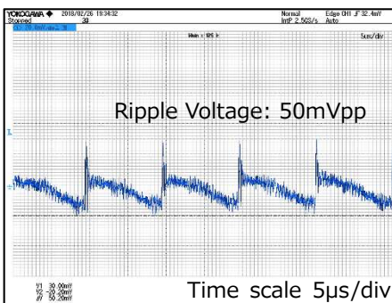
V_{IN}=230Vac, I_{OUT}=150mA
