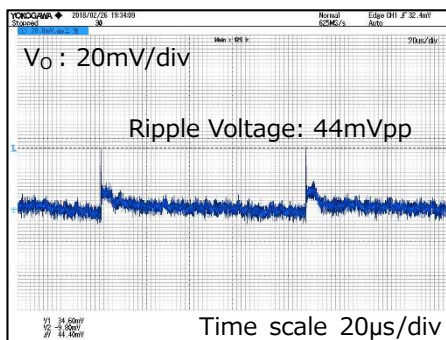
V_{IN}=230Vac, I_{OUT}=10mA
