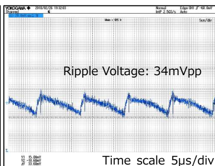
V_{IN}=100Vac, I_{OUT}=200mA
