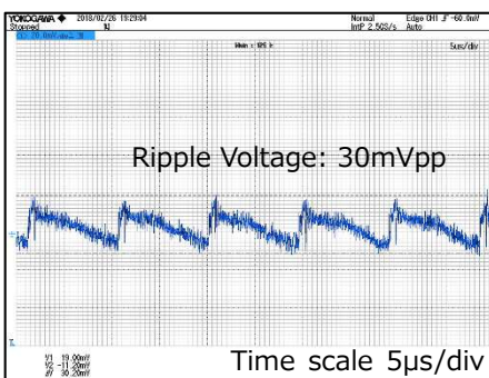
V_{IN}=100Vac, I_{OUT}=150mA
