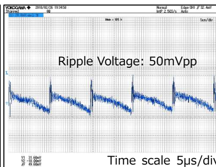
V_{IN}=230Vac, I_{OUT}=200mA
