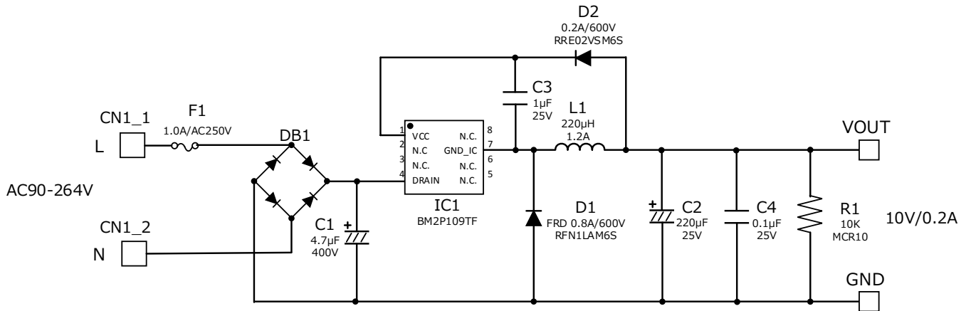
Figure 3. BM2P109TF-EVK-001 Schematics
