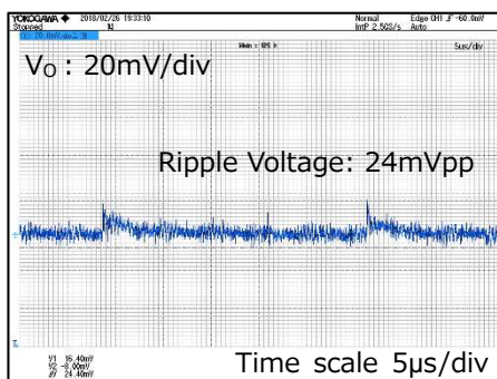
V_{IN}=100Vac, I_{OUT}=10mA
