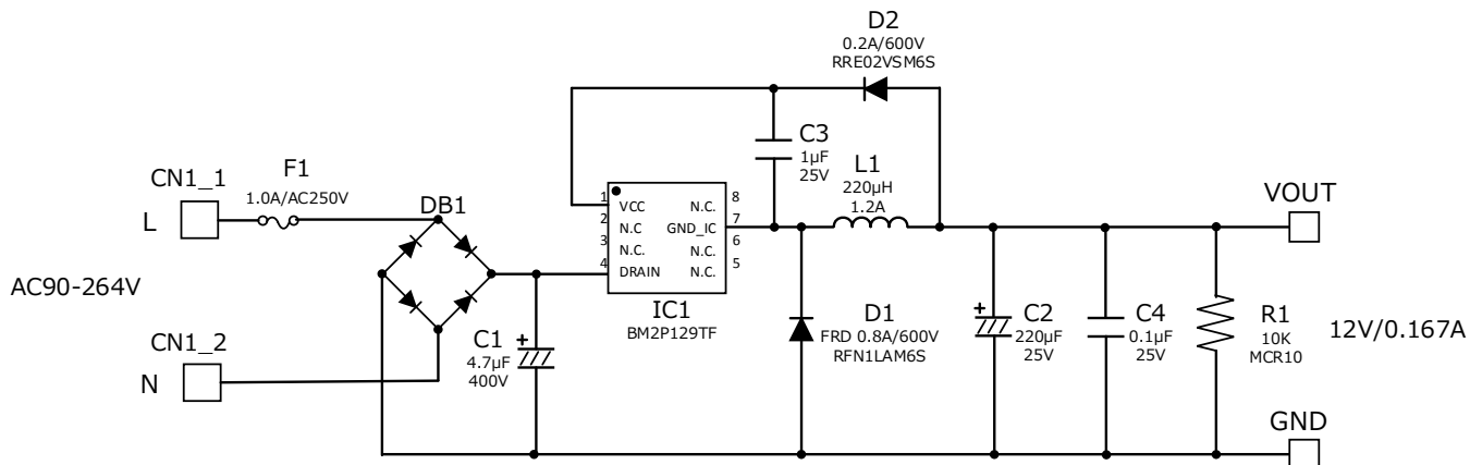
Figure 3. BM2P129TF-EVK-001 Schematics
