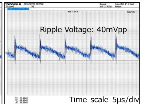
V_{IN}=230Vac , I_{OUT}=167mA
