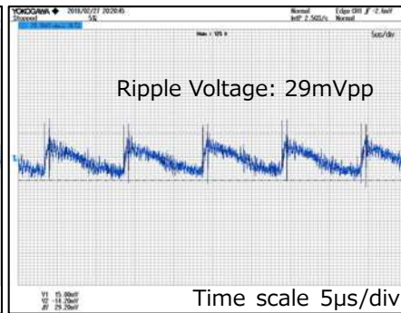
V_{IN}=100Vac , I_{OUT}=100mA
