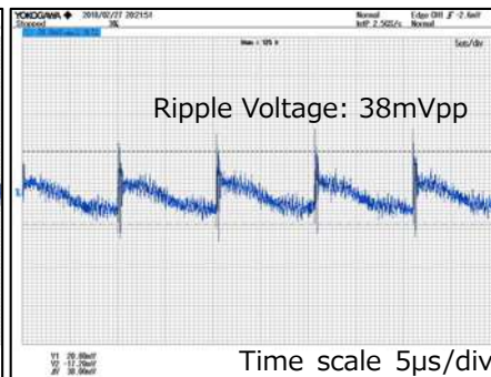
V_{IN}=230Vac , I_{OUT}=100mA
