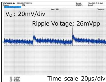
V_{IN}=230Vac , I_{OUT}=10mA
