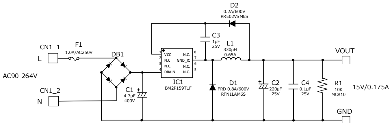
Figure 3. BM2P159T1F-EVK-001 Schematics
