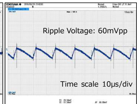
V_{IN}=100Vac, I_{OUT}=600mA
