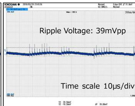
V_{IN}=100Vac, I_{OUT}=100mA
