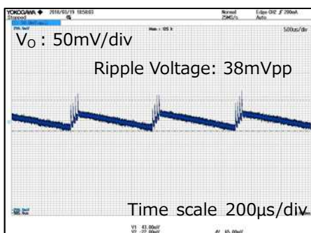
V_{IN}=230Vac, I_{OUT}=10mA
