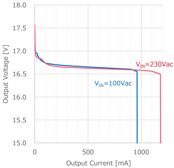
Figure 6. Load Regulation ( I_{OUT} vs. V_{OUT} )
