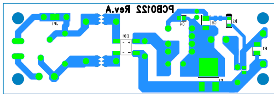
Figure 5. Bottom Layout (Top view)
