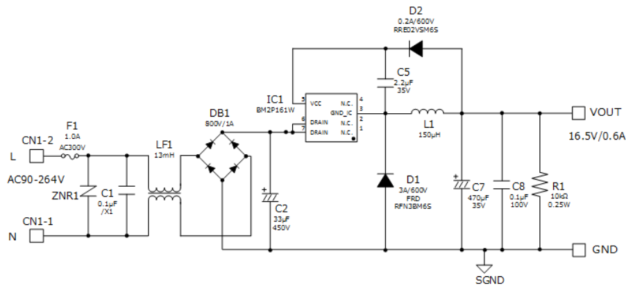
Figure 3. BM2P161W-EVK-001 Schematics
