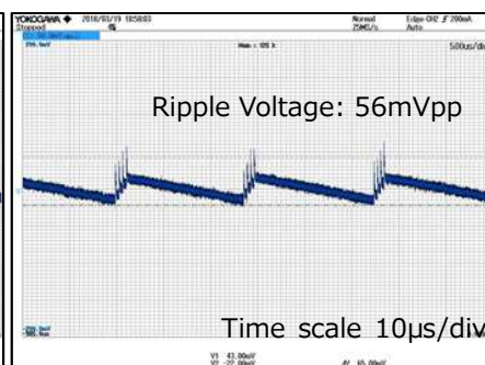
V_{IN}=230Vac, I_{OUT}=100mA
