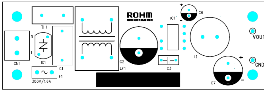
Figure 4. Top Silkscreen (Top view)
