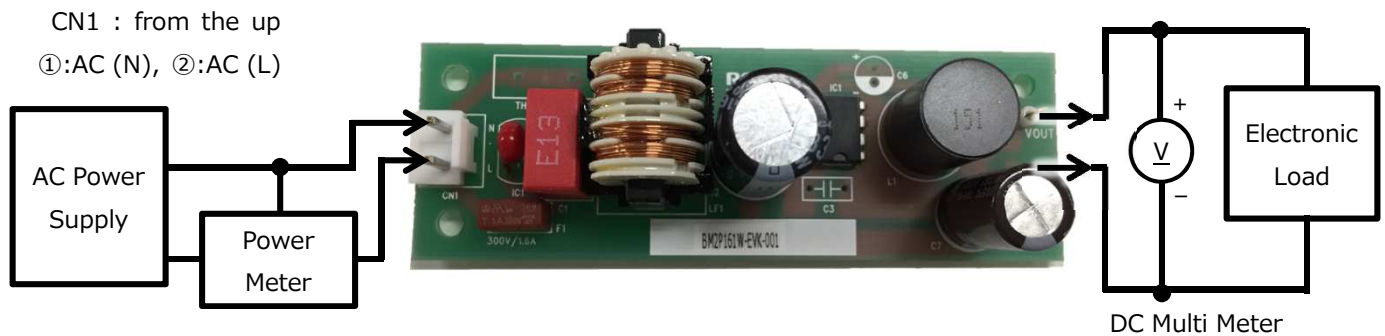
Figure 1. Connection Circuit
