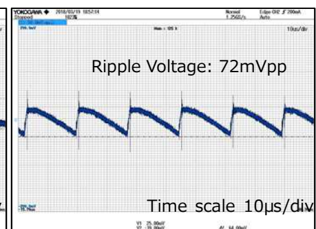
V_{IN}=230Vac, I_{OUT}=600mA
