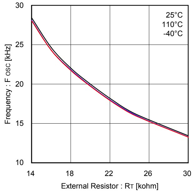
Figure 35. Carrier Frequency - RT
