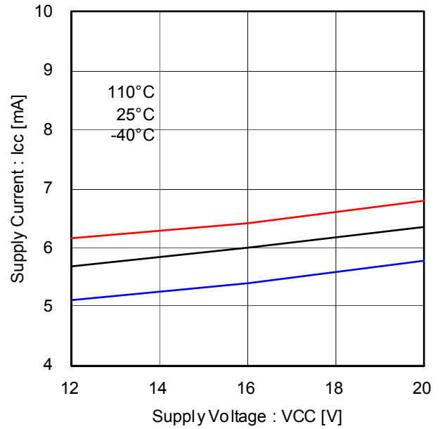
Figure 16. Low Side Drivers Operating Current (F PWM : 20kHz)
