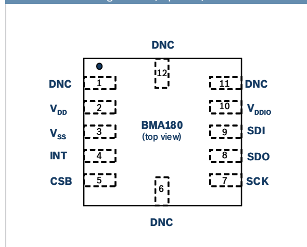
BMA180 Pin configuration (top view)
