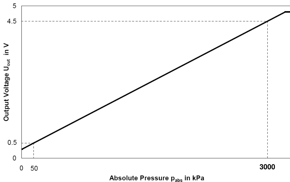
Figure 2. Characteristics at U_{\text{S}} = 5.000 V (schematic view)
