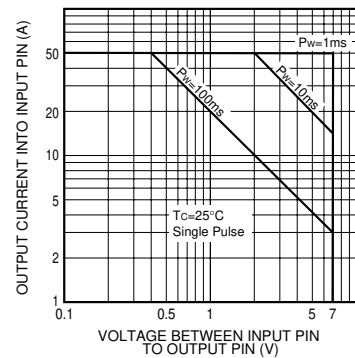
Fig.8 Safe operation range
