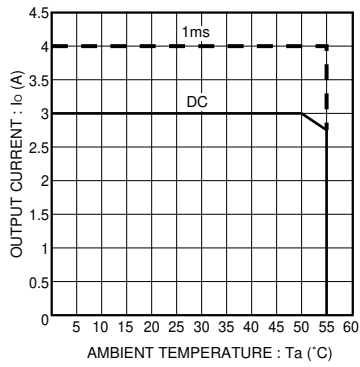
Fig.15 Derating curve
