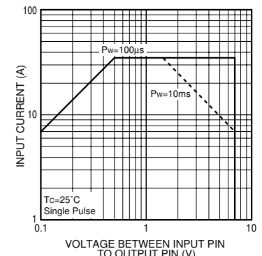
Fig.11 Safe operation range
