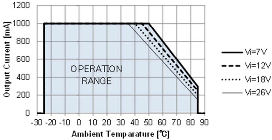
Fig.25 Derating curve(BP5293-33)
