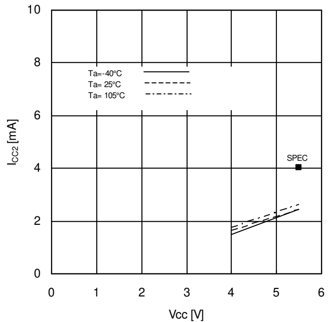
Figure 12. Supply Current (Read) vs Supply Voltage (f SK =10MHz)
