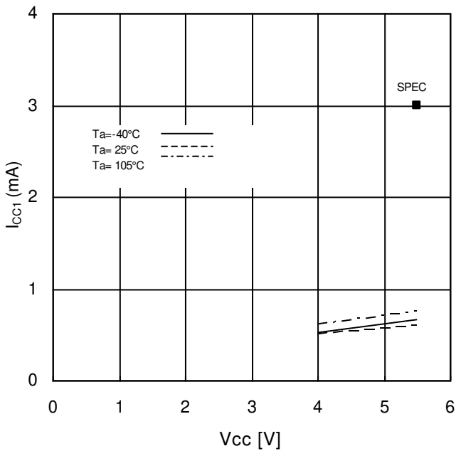
Figure 11. Supply Current (Write) vs Supply Voltage (f SK =10MHz)
