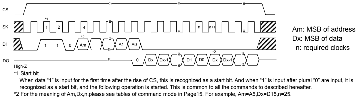
Figure 35. Read cycle
