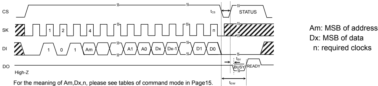
Figure 36. Write cycle
