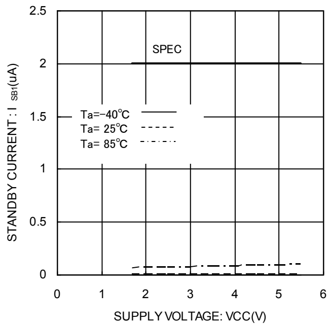
Figure 19. Standby current I_sbr1(CS=0V, ORG=VCC or OPEN)
