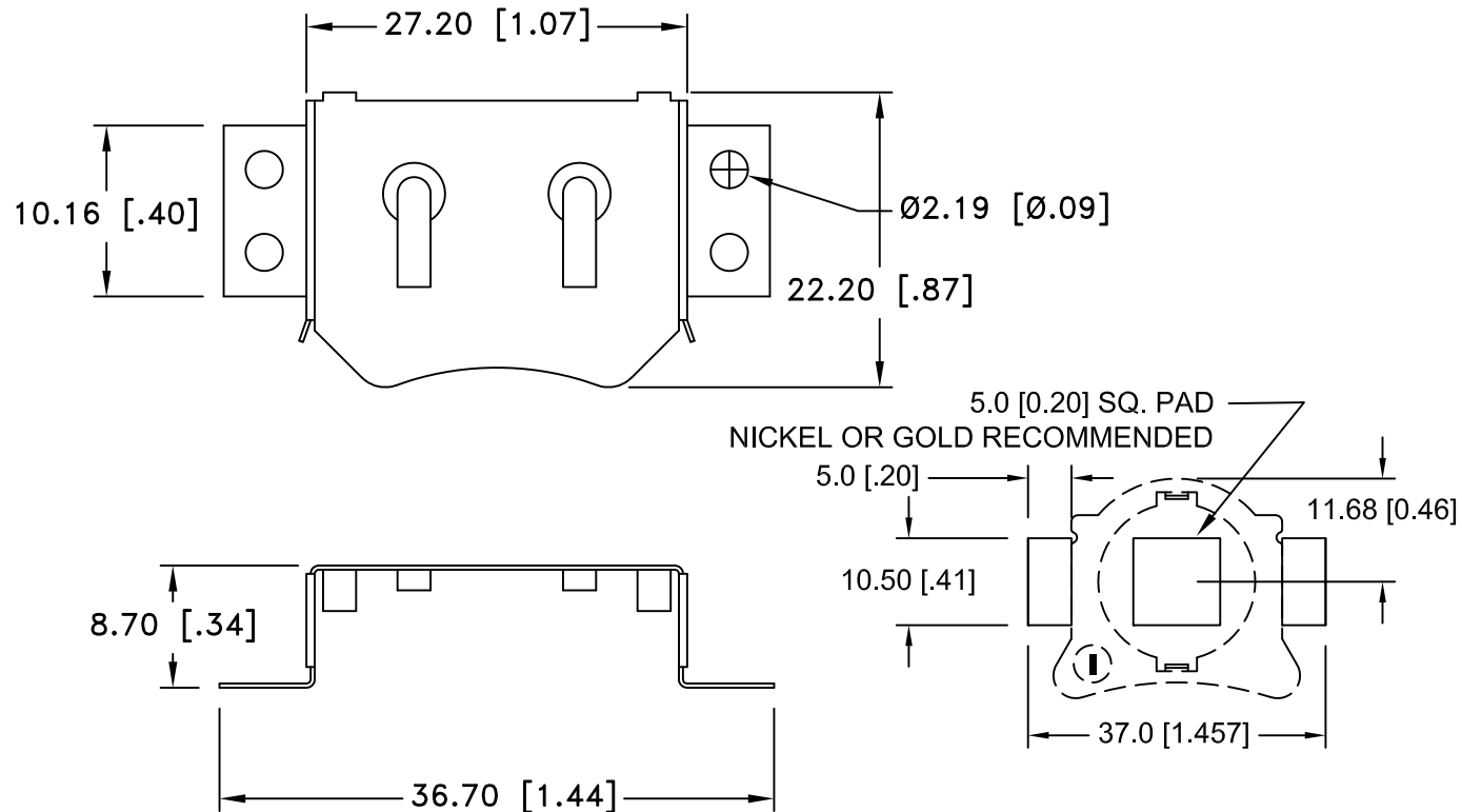
PCB LAYOUT
