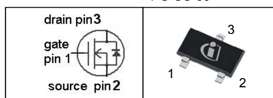
PG-SC-59
