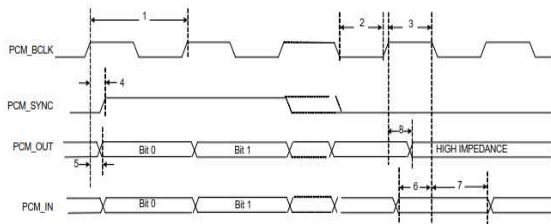
Figure 4: PCM timing diagram (Long-Frame Sync, Master Mode)
