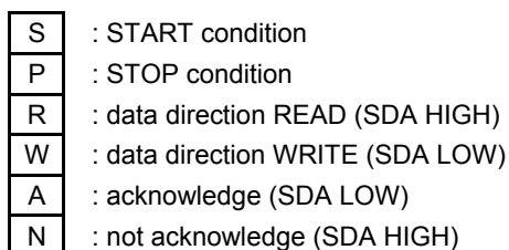
Figure 7. Read/Write Protocol
